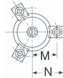
Bushing 3 Clamp Arrangement
